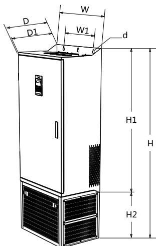
Figure 2-1-3 Outline dimension diagram 3
